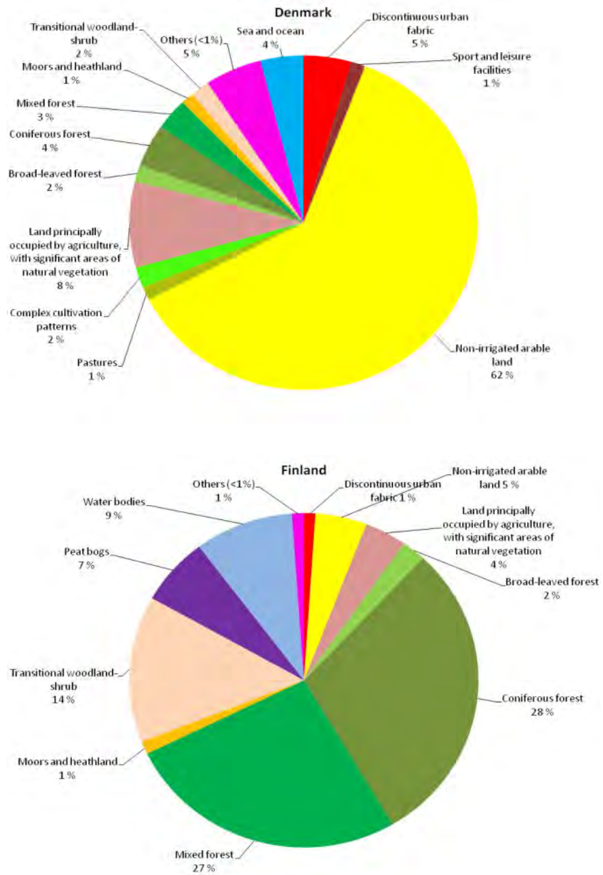
Figure 7.3 a-e: Main land cover types of the Nordic countries. The classes of which share of the total land cover were less than 1% are summed together to the class “others”
